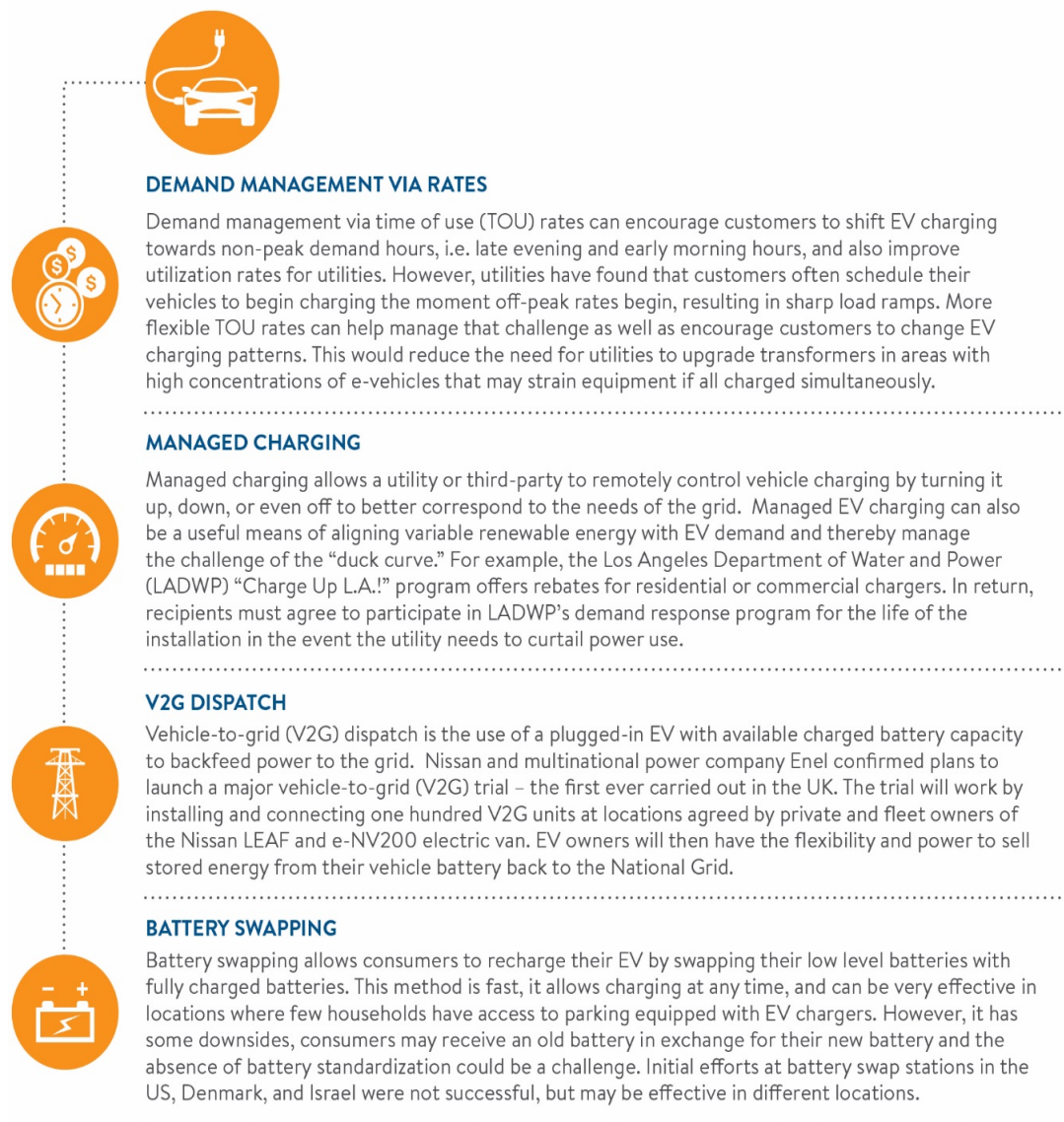
FIGURE 15: Integrating EVs as DERs into the power system
